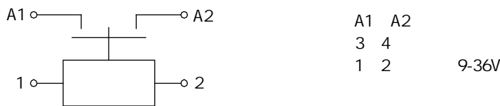
Wiring Diagram without Auxiliary Contact
